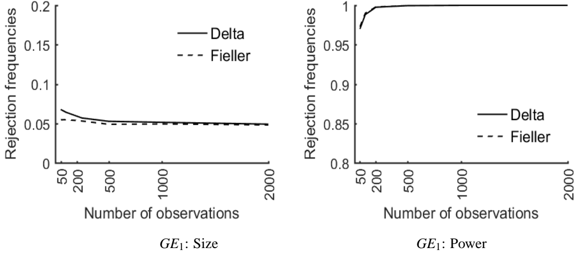
Figure 7: Design (I-c) – Size and power of Delta and Fieller-type tests for GE_1 comparisons
