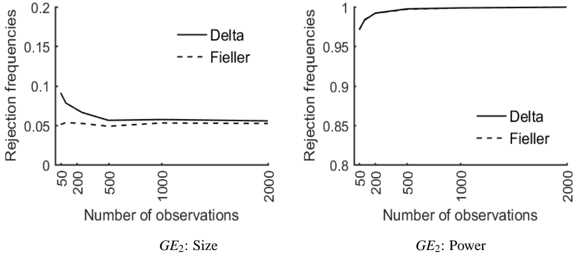
Figure 8: Design (I-c) – Size and power of Delta and Fieller-type tests for GE_2 comparisons
