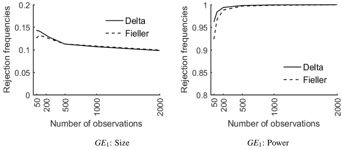
Figure 5: Design (I-b) – Size and power of Delta and Fieller-type tests for GE_1 comparisons
